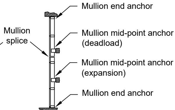
Multi-Span
