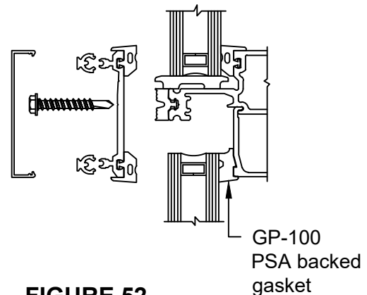
FIGURE 52 Outside Glazed Horizontal Reglazing
