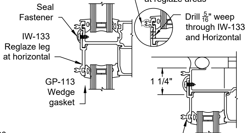
FIGURE 50 Reglazing
