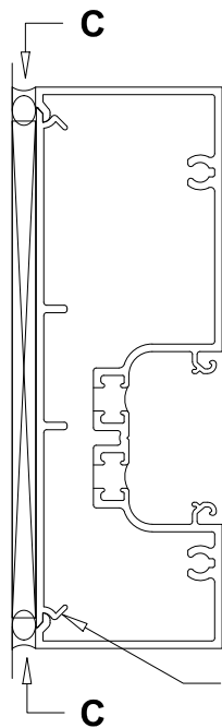
FG-6188 optional PVC filler for sealant backer
