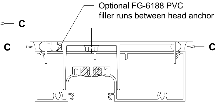
FG-6431-01 head anchor for center set system only Maximum end reaction is 600 lbs
