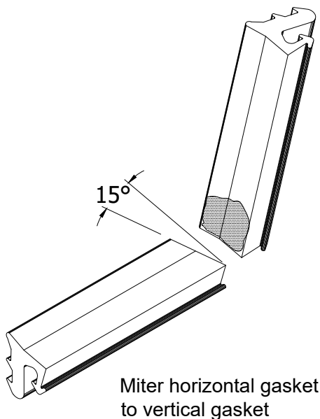
DETAIL "A"
