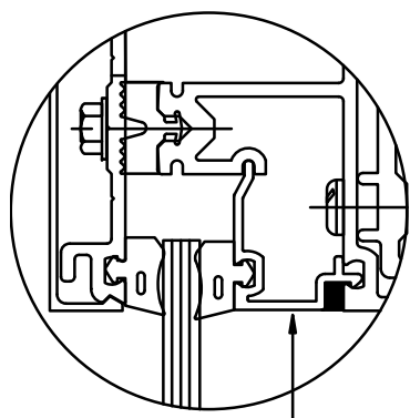
WW-130 ADAPTOR SEALED CONTINUOUS
