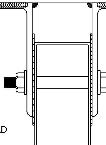
Plan View Intermediate Mullion
