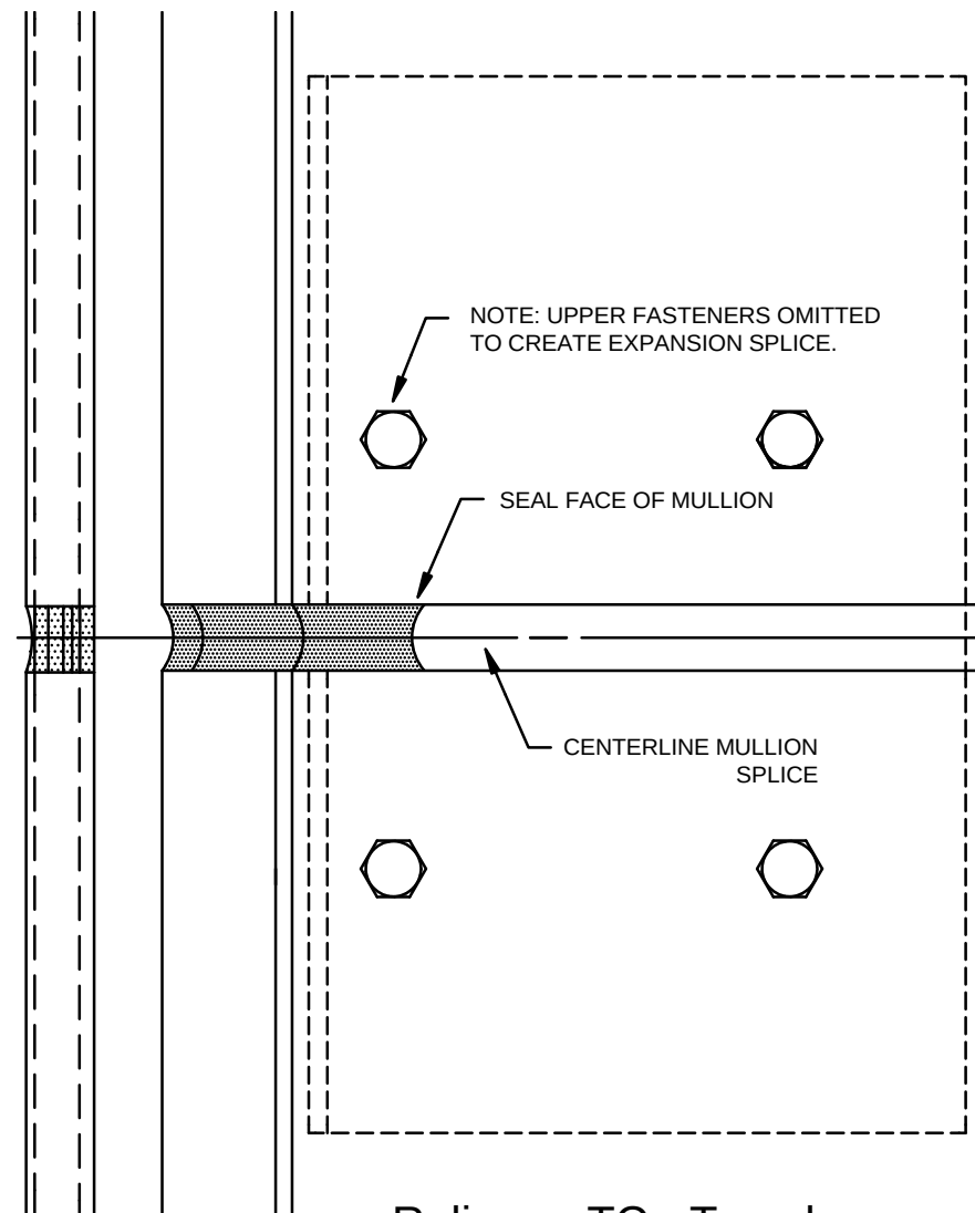
Reliance-TC - Type I Corner Mullion Splice - H7444
