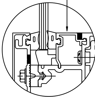
WW-130 ADAPTOR & GP-110 SETTING BLOCK
