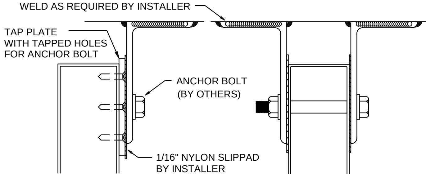
Plan View Jamb Option
