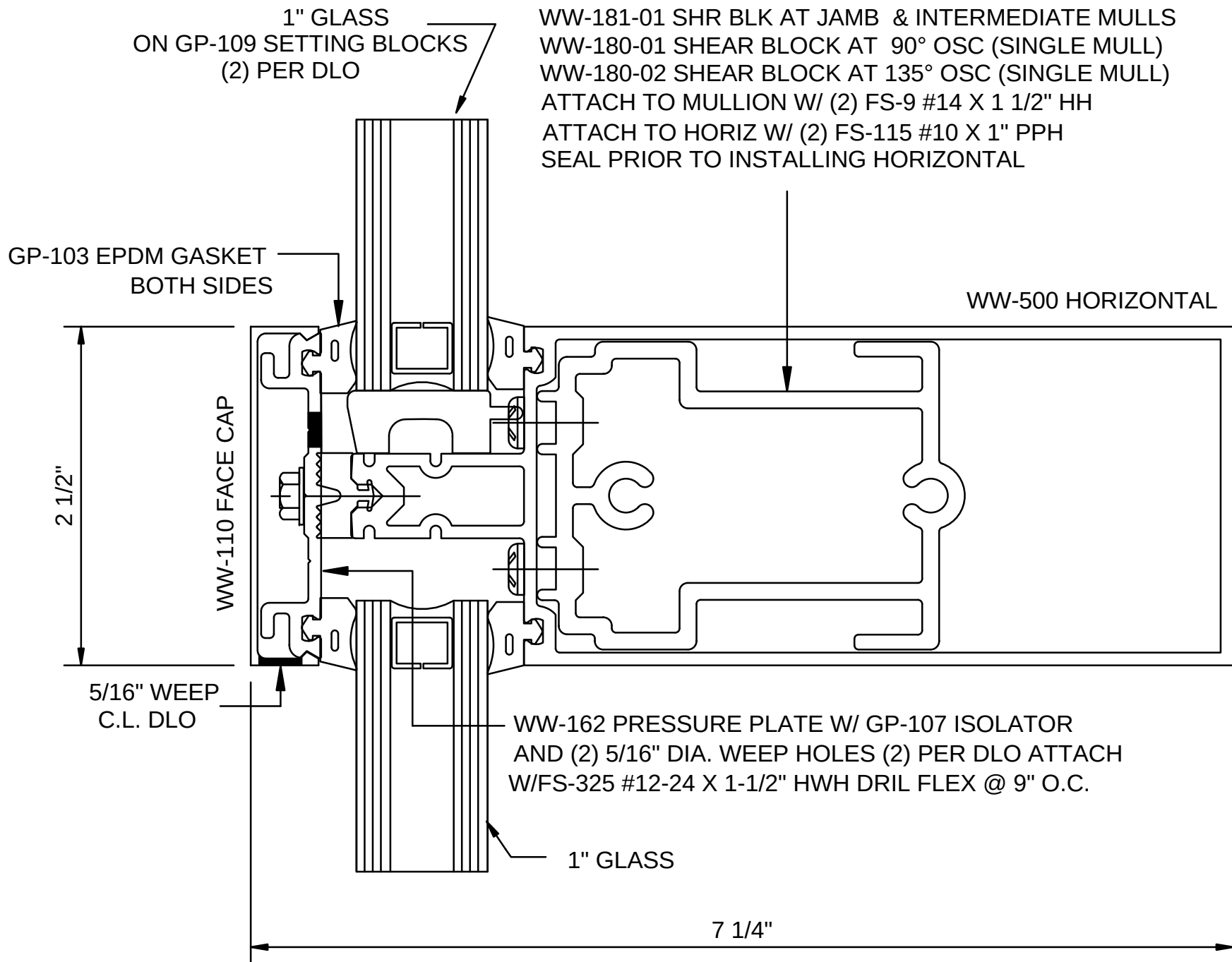
Reliance - Standard Horizontal at Vison - H3405
