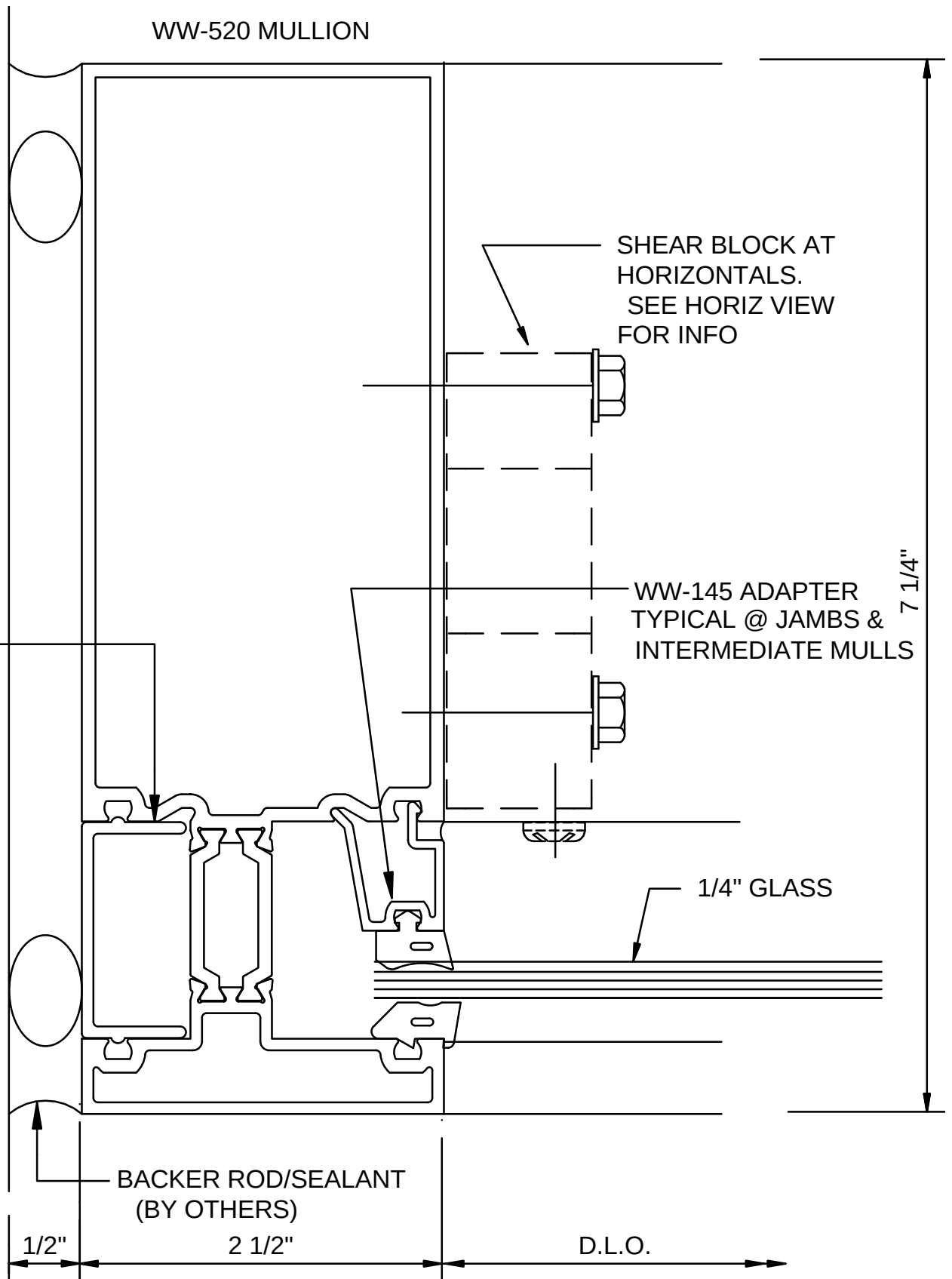
Reliance -TC - Type I Jamb @ Spandrel - V7403
