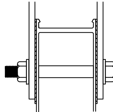
Plan View Inside - Outside Corner
