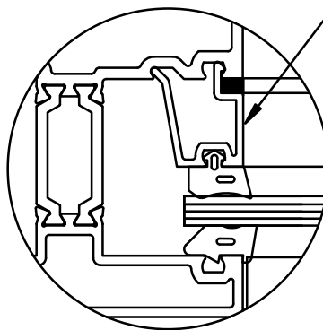
WW-145 GLAZING ADAPTOR SET IN SEALANT
