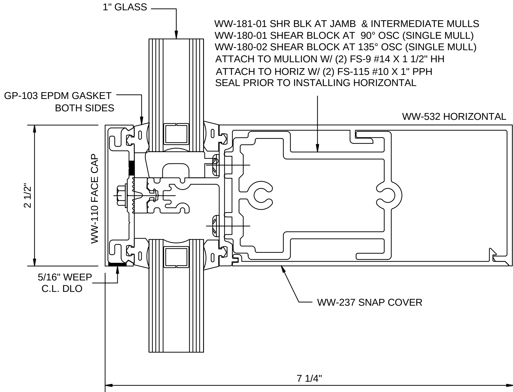
Reliance - Roll Over Horizontal - H3408
