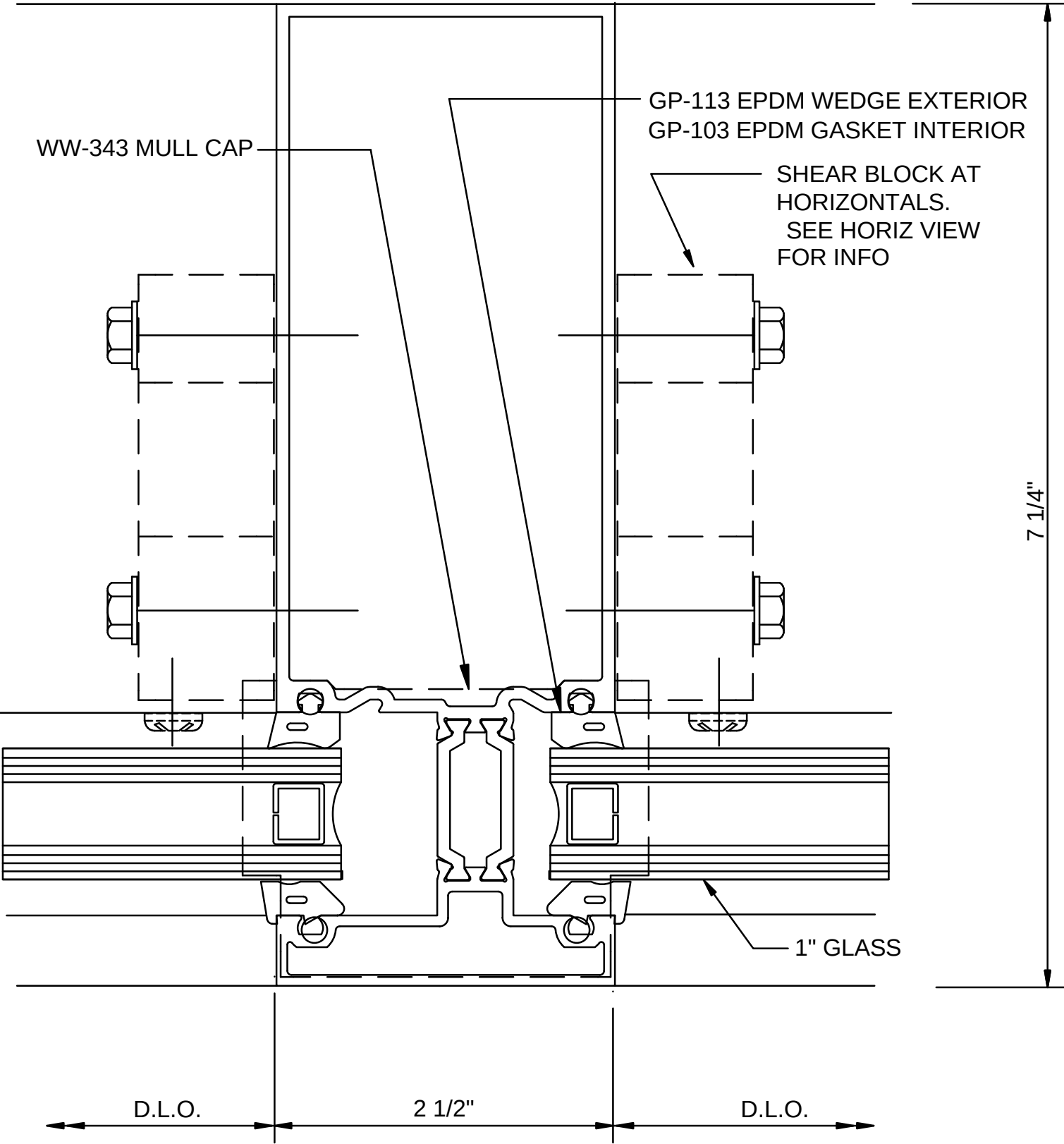
Reliance -TC - Type I Vertical Mullion - V7402
