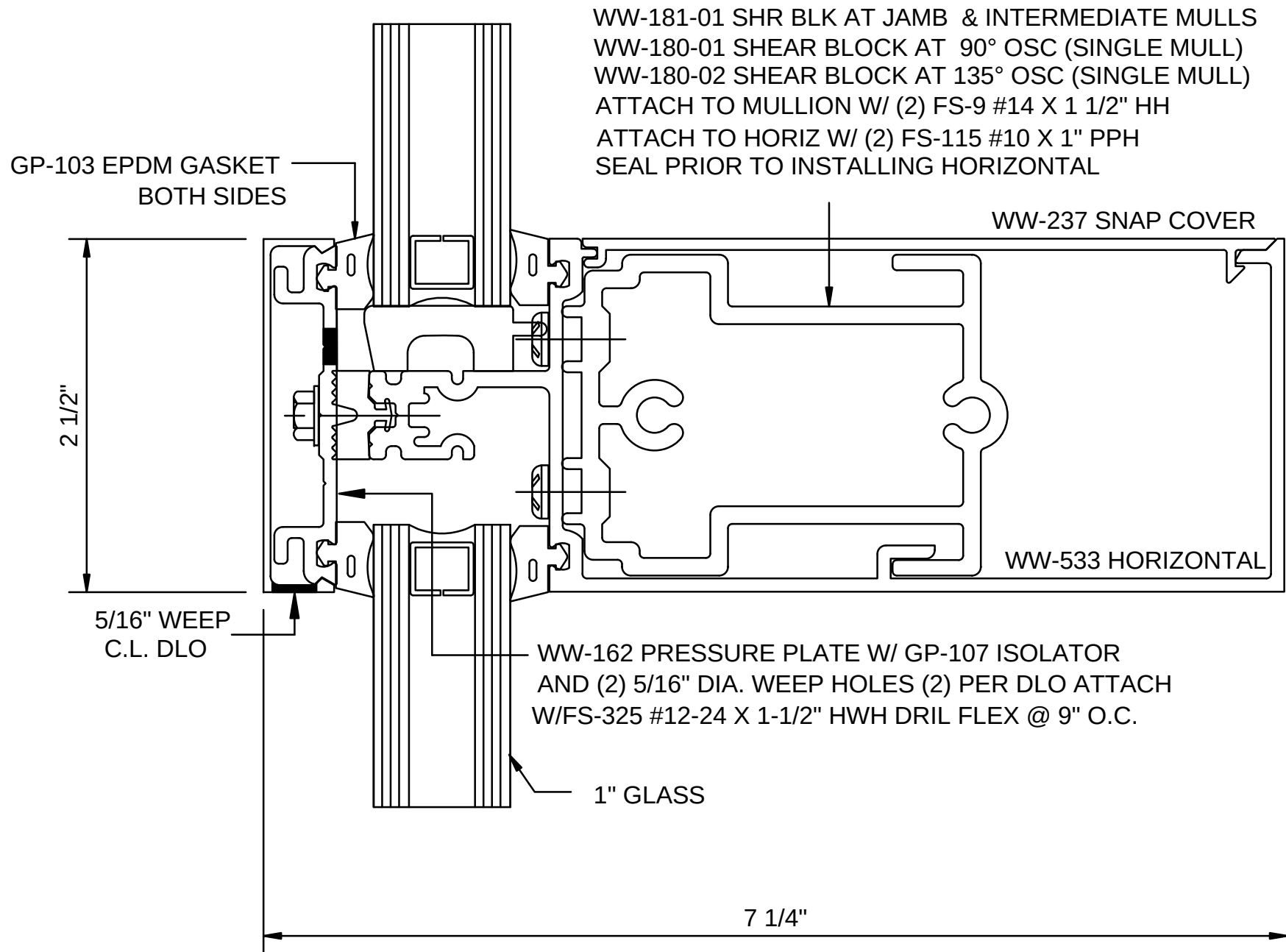
Reliance - Roll Under Horizontal - H3409
