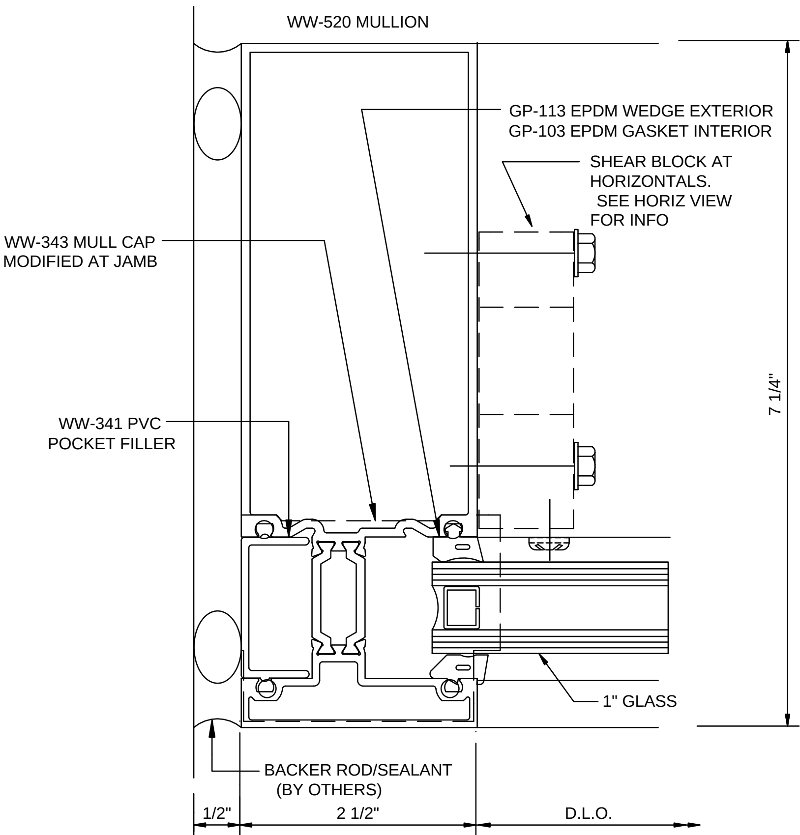
Reliance -TC - Type I Jamb Mullion - V7401
