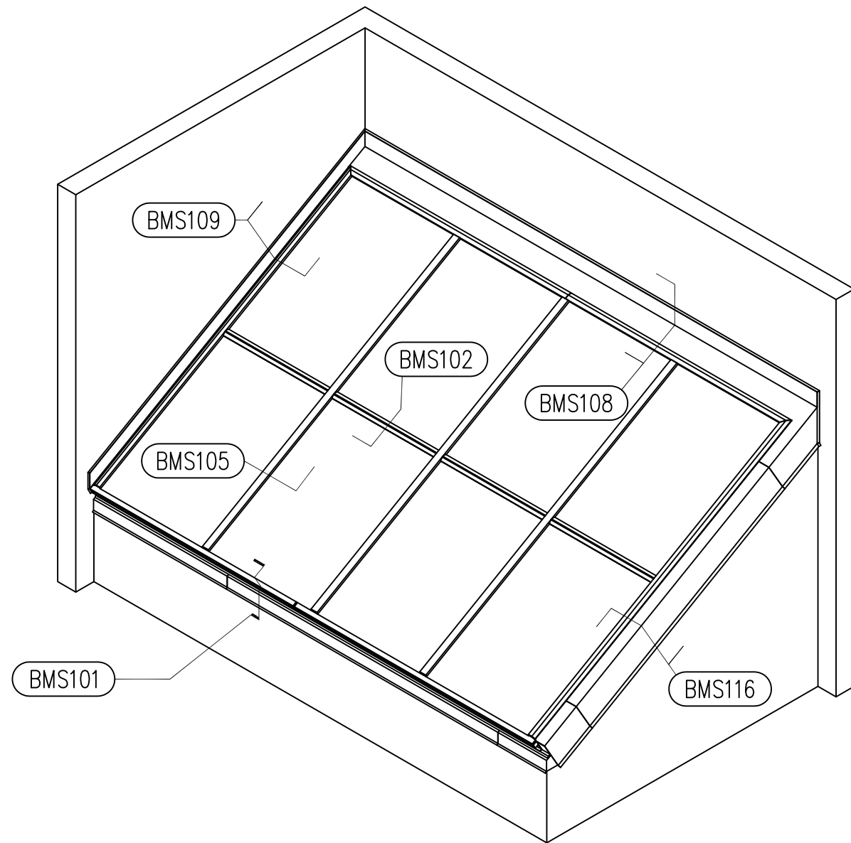
ISOMETRIC VIEW OF SINGLE SLOPE SKYLIGHT
