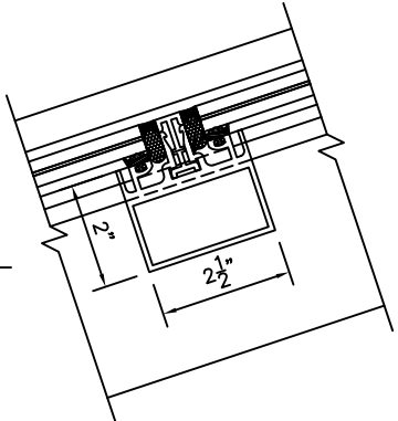
BMS103 PURLIN 2-SIDED SILICONE GLAZED OPTION FOR LOW SLOPES
