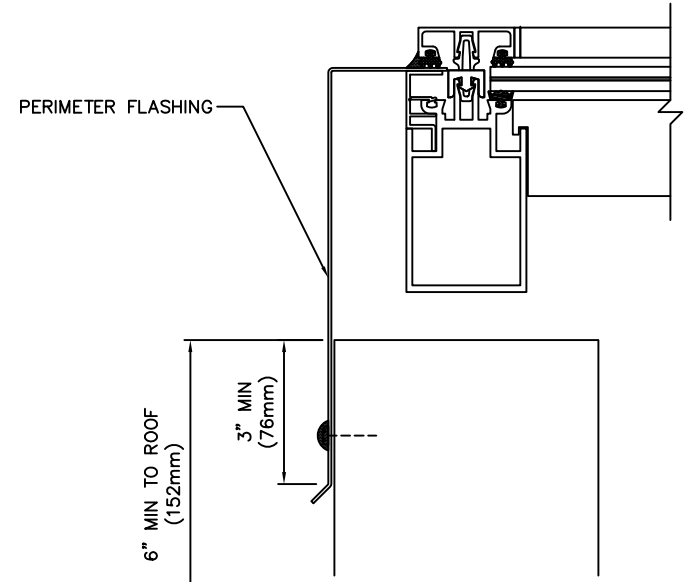
BMS116 END RAFTER @ ROOF CURB OR PARAPET WALL
