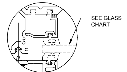
90° OUTSIDE CORNER
