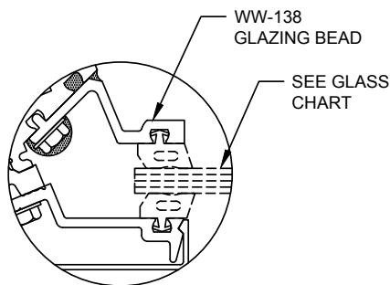
135° INSIDE CORNER (SEE NOTE 5)
