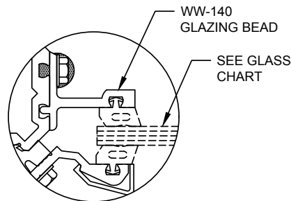
90° INSIDE CORNER (SEE NOTE 5)
