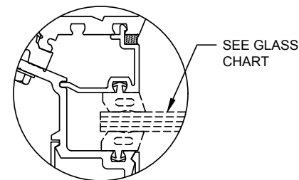
135° OUTSIDE CORNER
