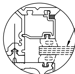
90° OUTSIDE CORNER
