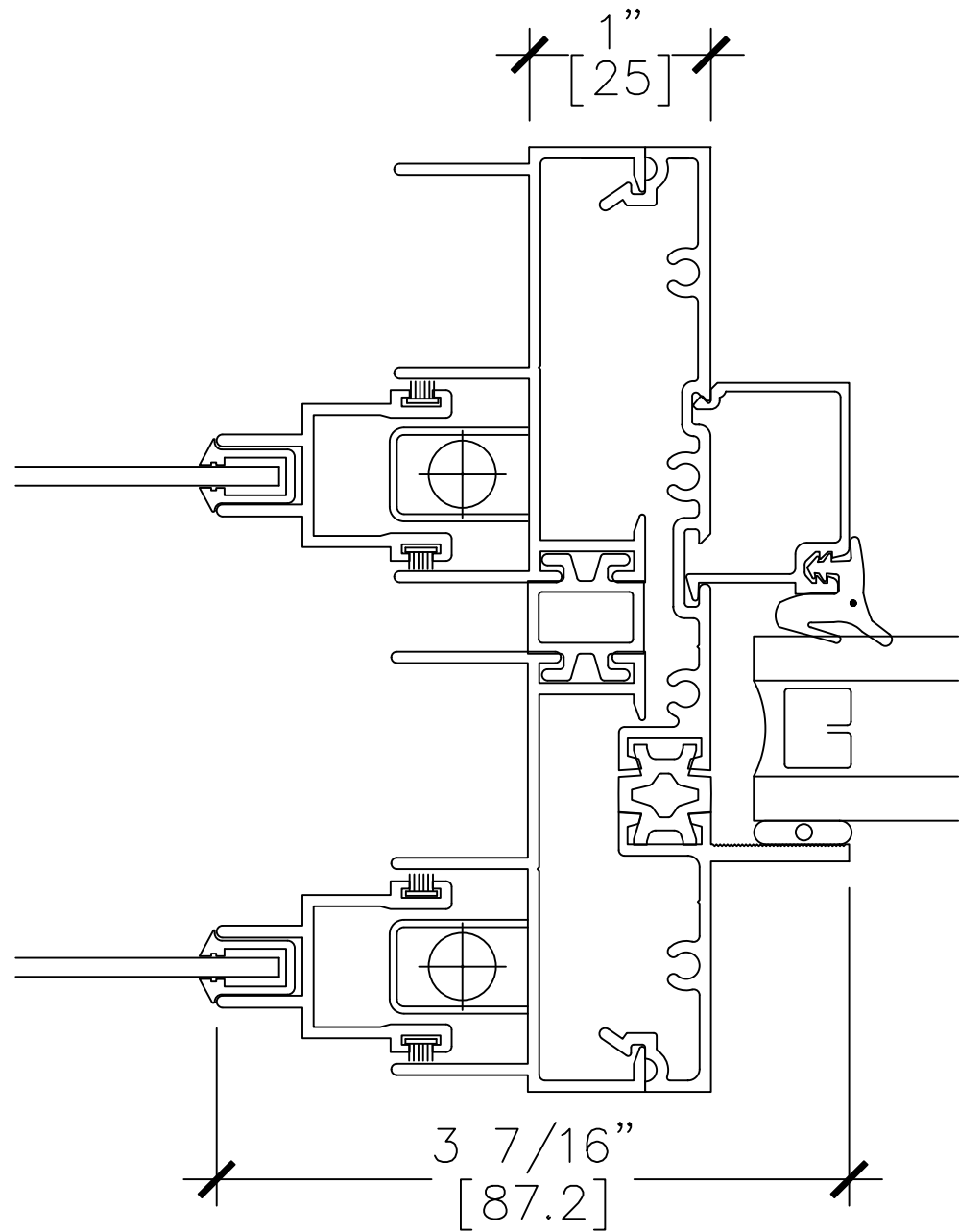
14 Double Hung Beside Fixed Upper Sash Vertical Snap
