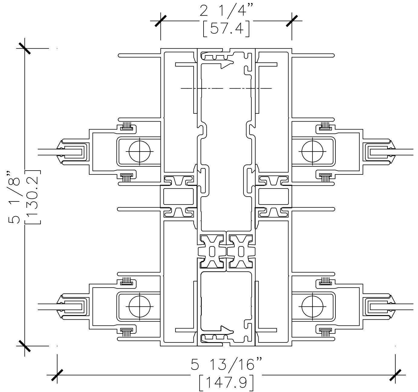
14 Operable Sash with Double Split Mullion
