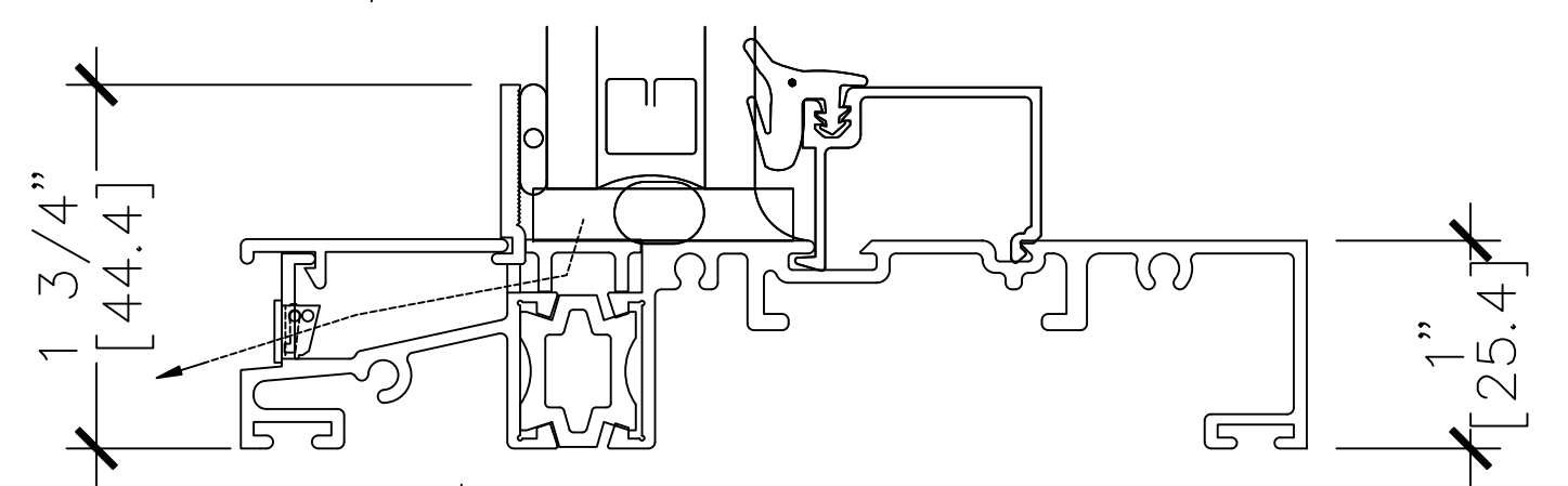
20 Fixed Sill Detail [ Rainscreen Sill ]
