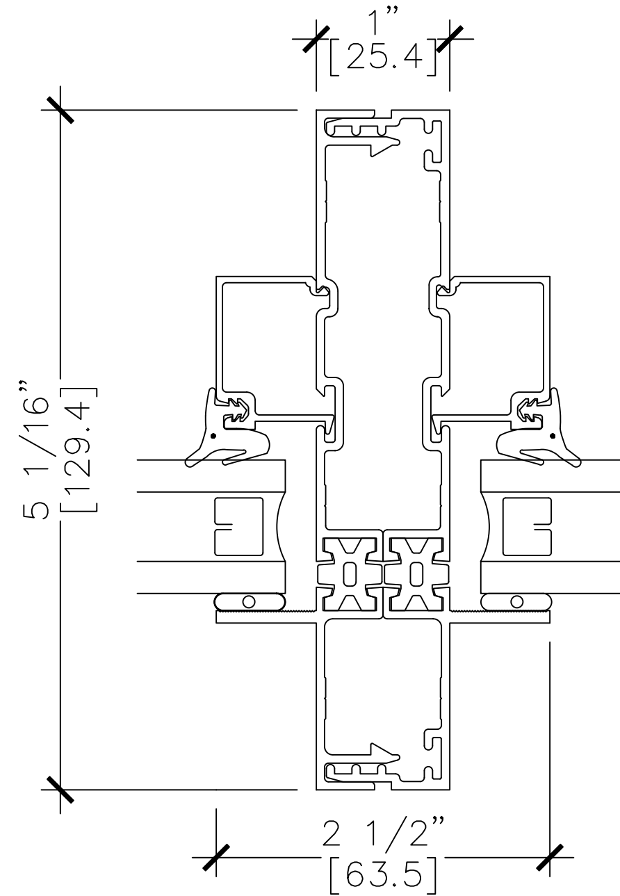
13 1" Split Mullion Fixed Sash
