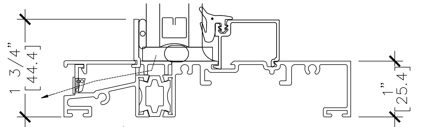
20 Fixed Sill Detail [ Rainscreen Sill ]
