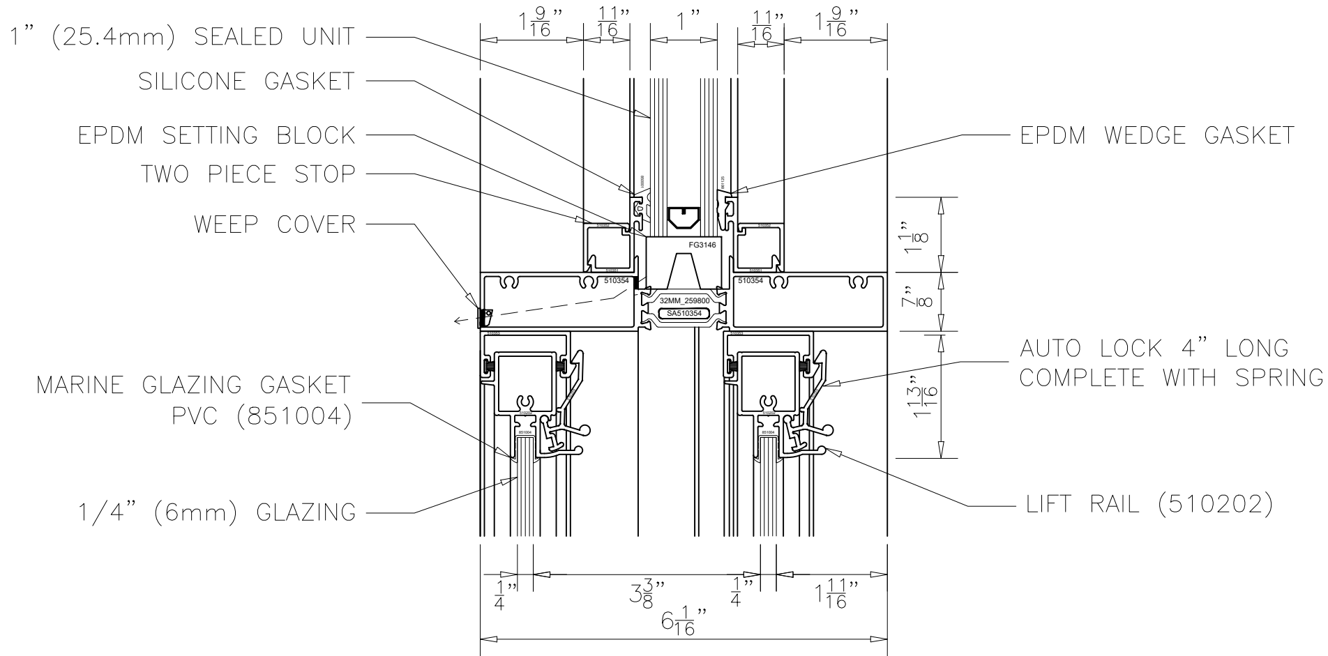
DOUBLE HUNG OPERABLE WINDOW 5100 6AR SERIES HEAD TRANSOM SILL SCREEN BETWEEN SASH
