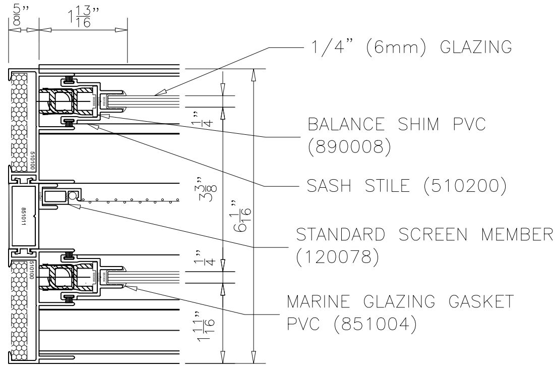
DOUBLE HUNG OPERABLE WINDOW 5100 6AR SERIES JAMB SCREEN BETWEEN SASH
