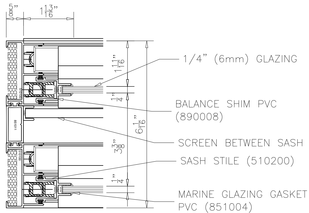
DOUBLE HUNG OPERABLE WINDOW 5100 6AR SERIES JAMB SCREEN BETWEEN SASH
