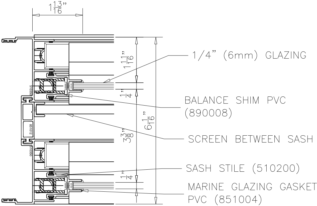
DOUBLE HUNG OPERABLE WINDOW 5100 6AR SERIES MALE SPLIT SCREEN BETWEEN SASH
