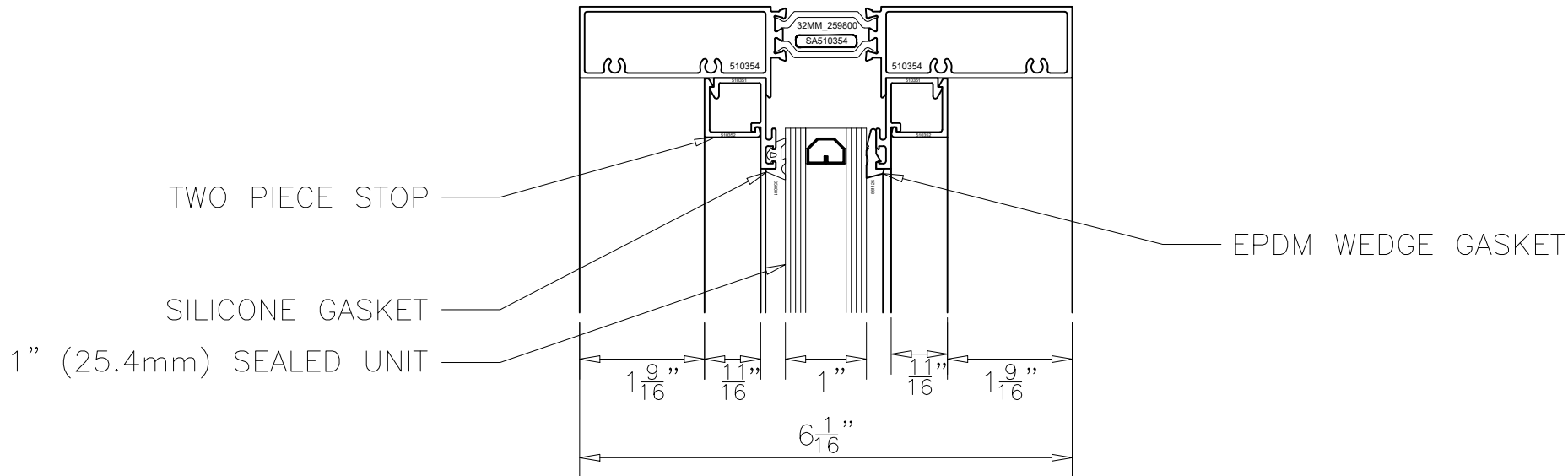
DOUBLE HUNG OPERABLE WINDOW 5100 6AR SERIES HEAD TRANSOM HEAD
