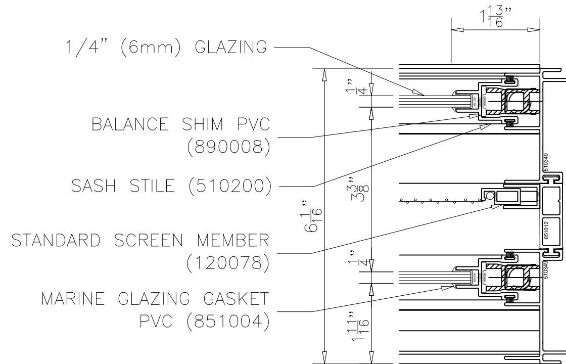
DOUBLE HUNG OPERABLE WINDOW 5100 6AR SERIES FEMALE SPLIT SCREEN BETWEEN SASH
