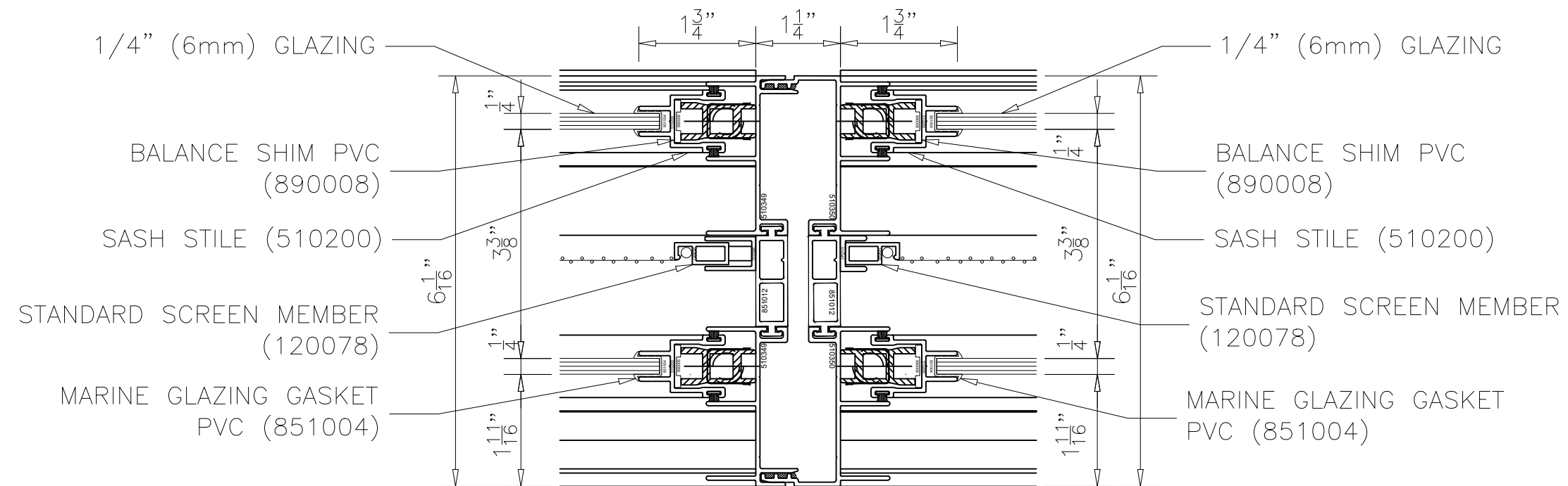
DOUBLE HUNG OPERABLE WINDOW 5100 6AR SERIES SPLIT MULLION SCREEN BETWEEN SASH
