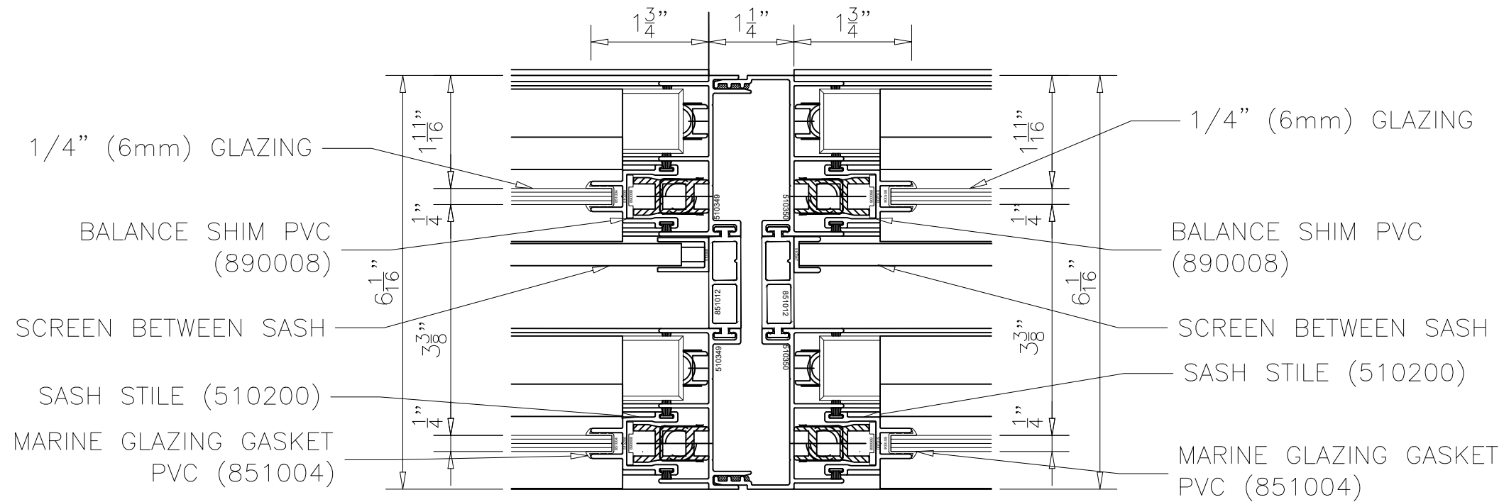
DOUBLE HUNG OPERABLE WINDOW 5100 6AR SERIES SPLIT MULLION SCREEN BETWEEN SASH
